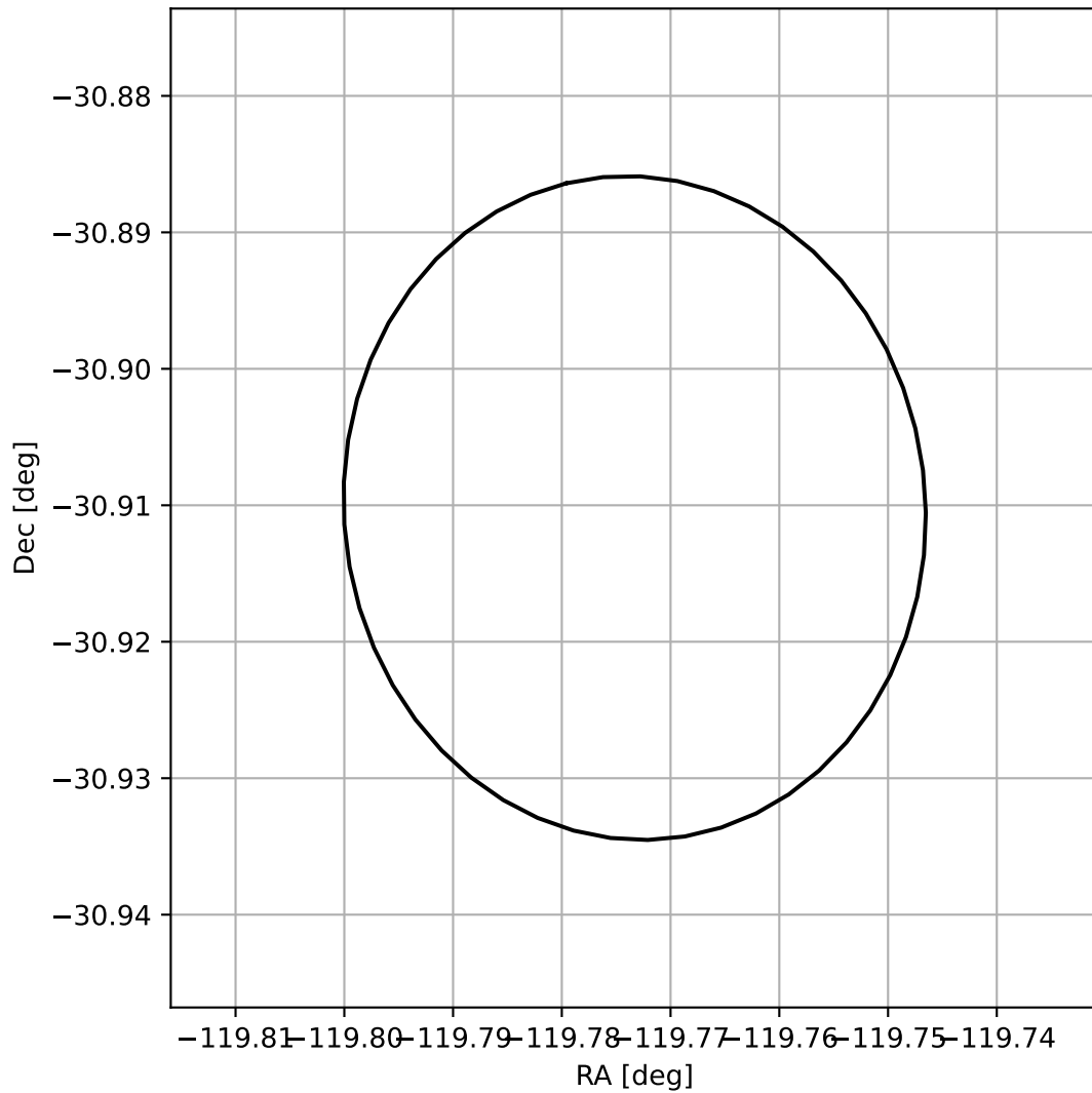
4FGL J1600.9-3054
