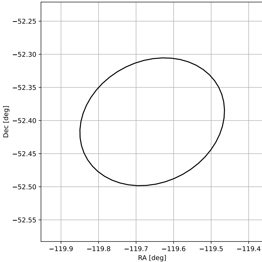
4FGL J1601.3-5224
