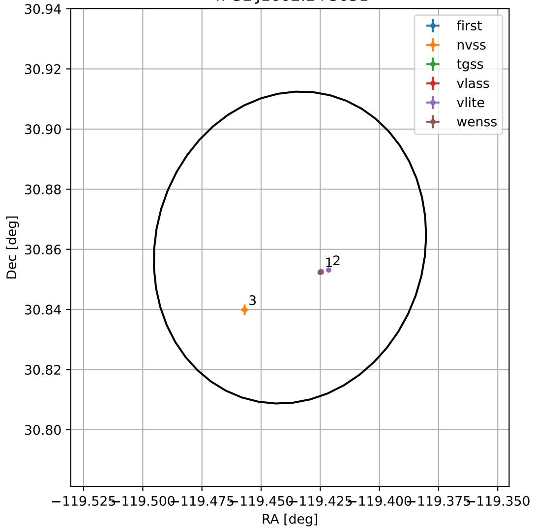
4FGL J1602.2+3051
