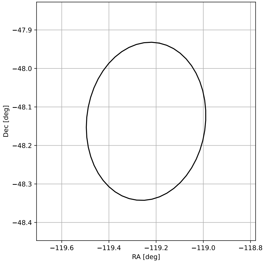
4FGL J1603.0-4808
