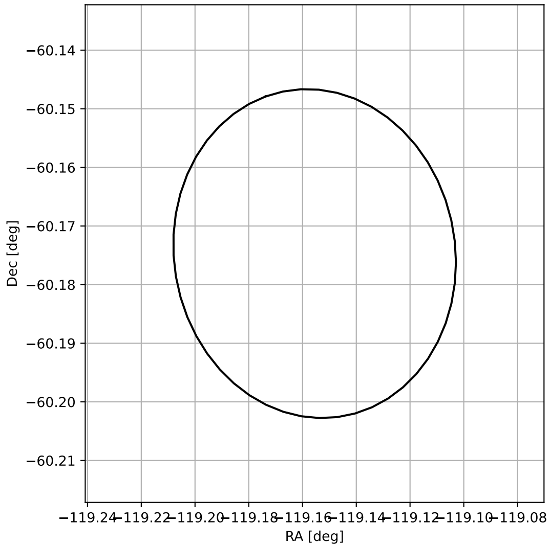
4FGL J1603.3-6010
