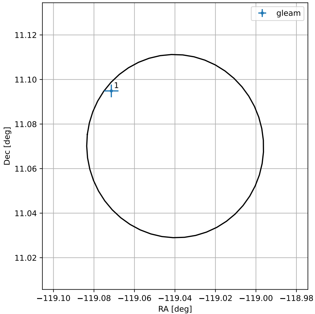
4FGL J1603.8+1104
