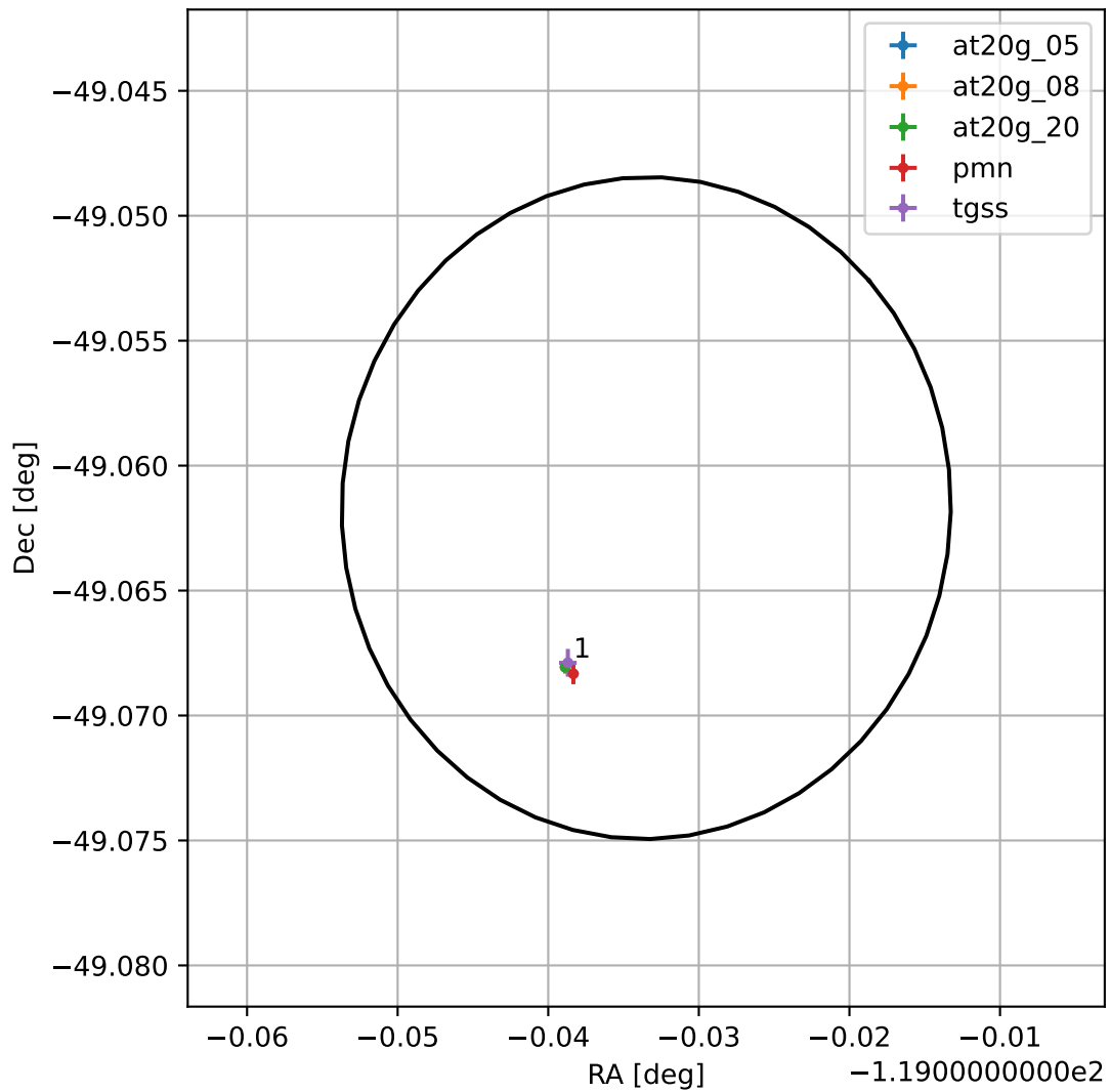
4FGL J1603.8-4903
