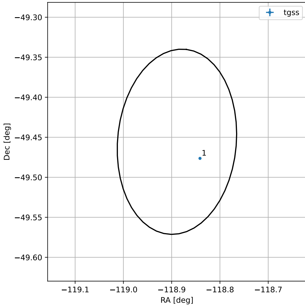
4FGL J1604.4-4927
