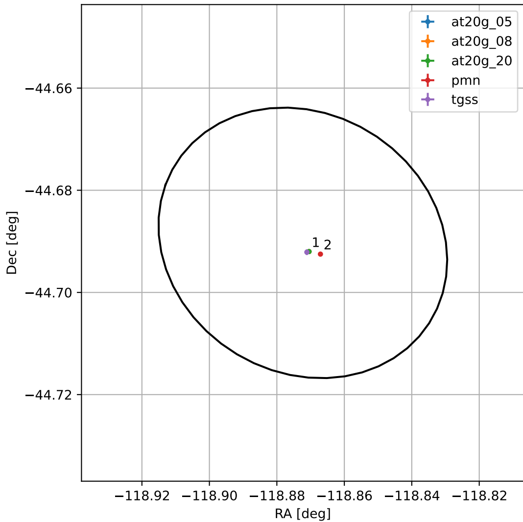
4FGL J1604.5-4441
