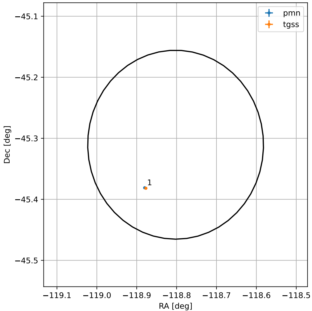
4FGL J1604.7-4518
