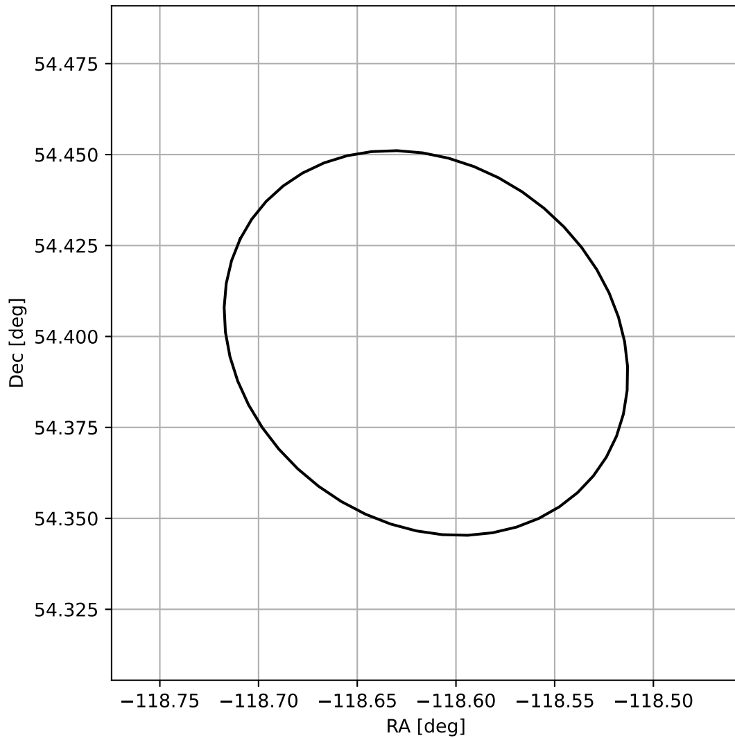
4FGL J1605.5+5423
