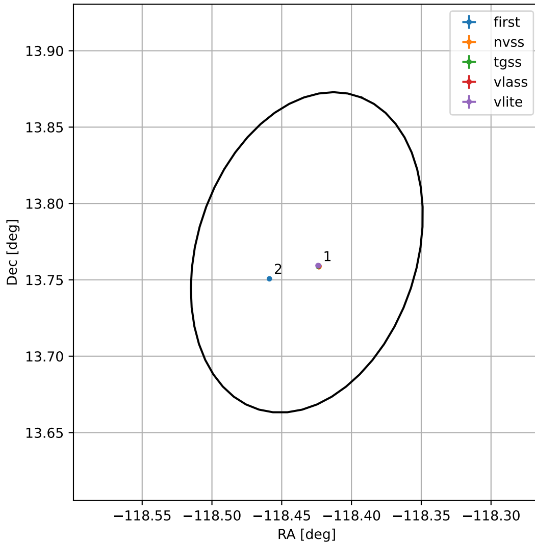
4FGL J1606.2+1346
