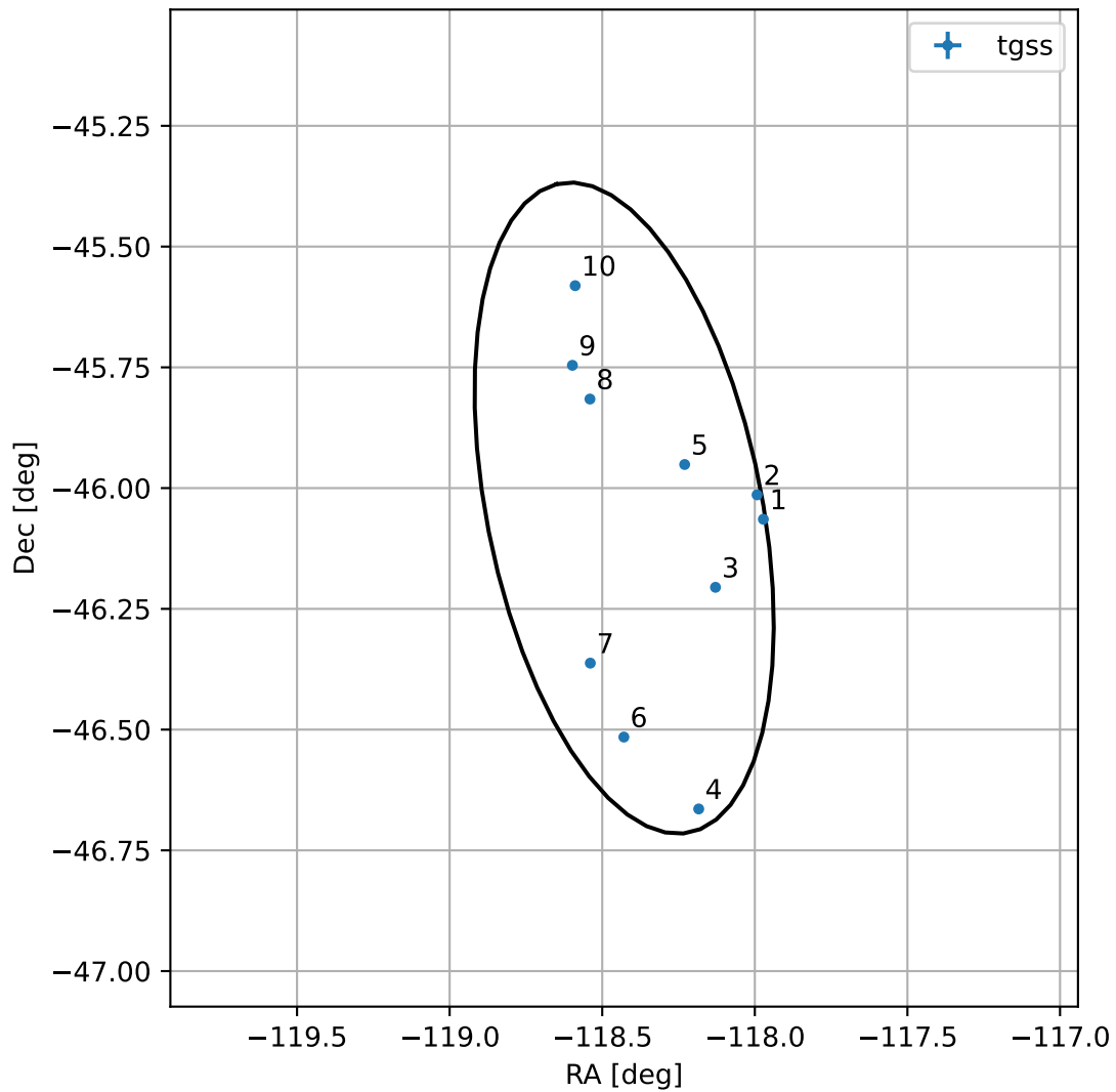
4FGL J1606.2-4602
