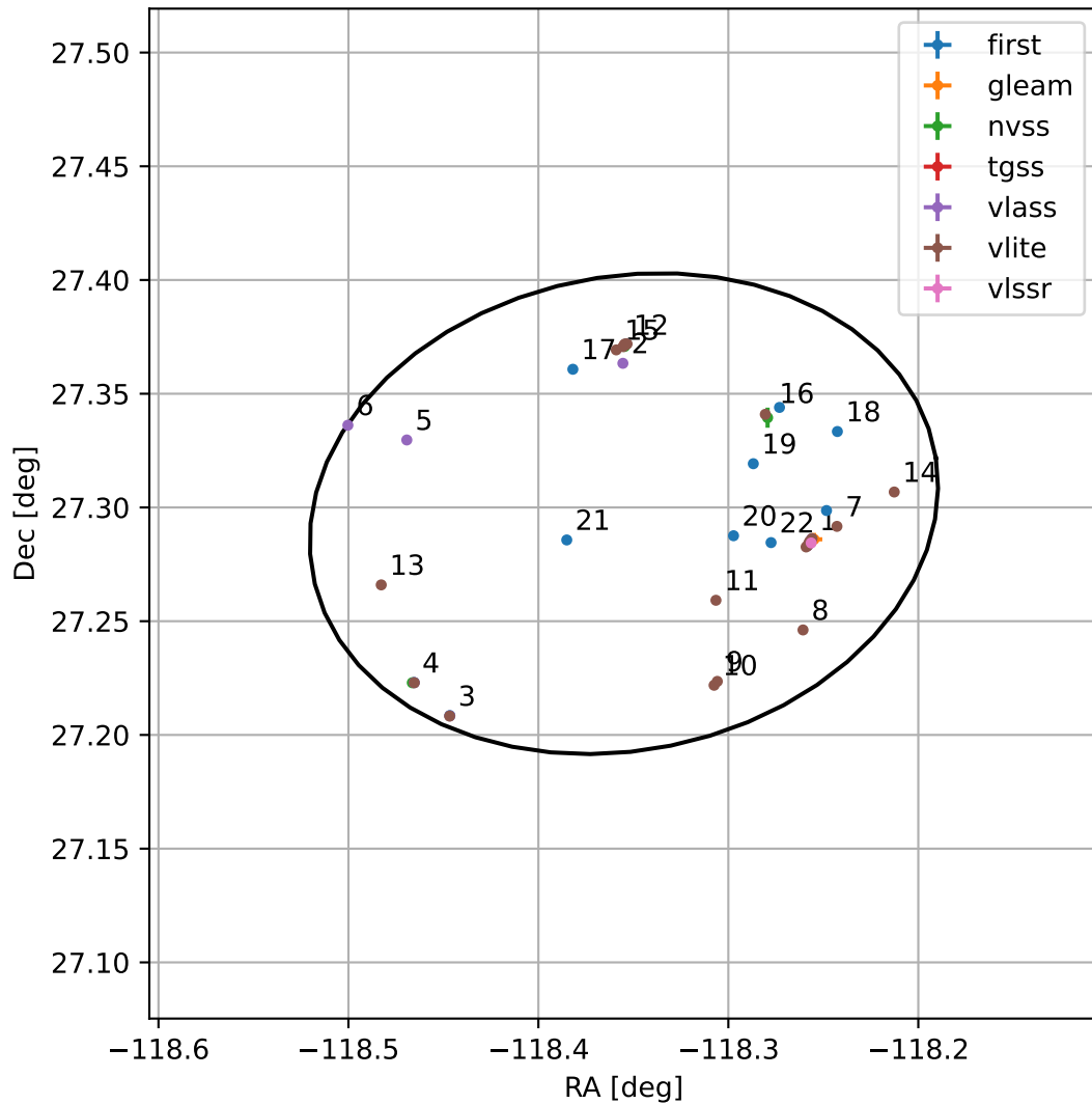
4FGL J1606.5+2717
