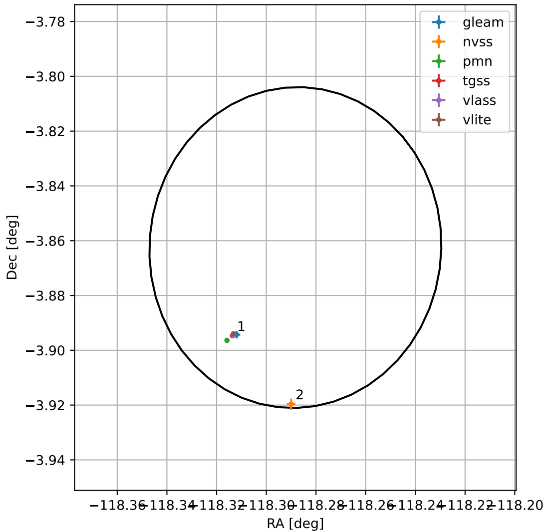
4FGL J1606.8-0351
