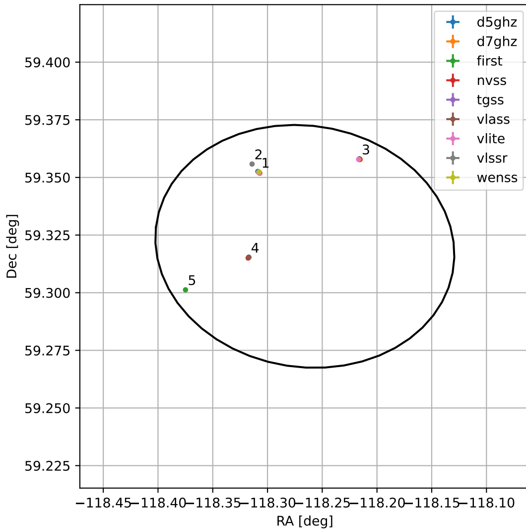
4FGL J1606.9+5919
