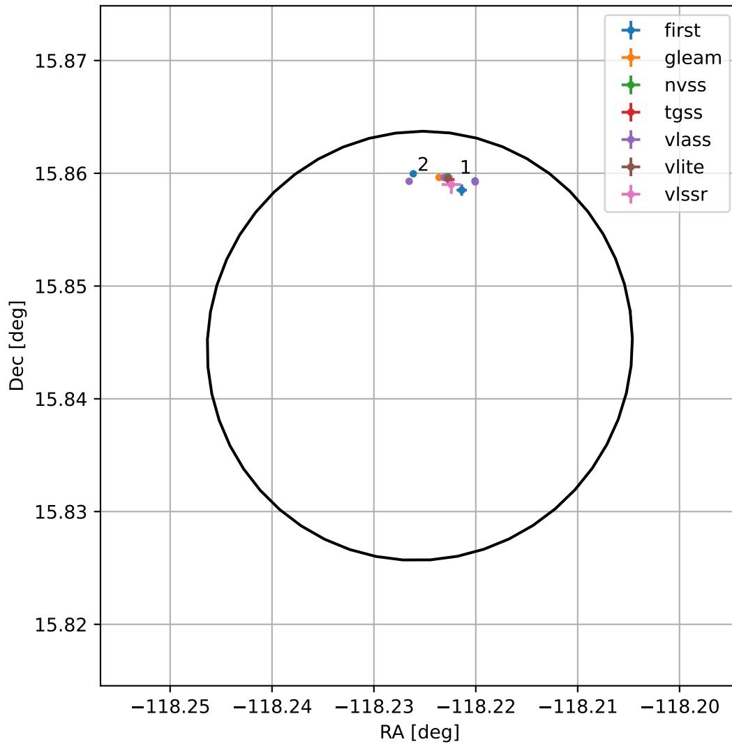
4FGL J1607.0+1550
