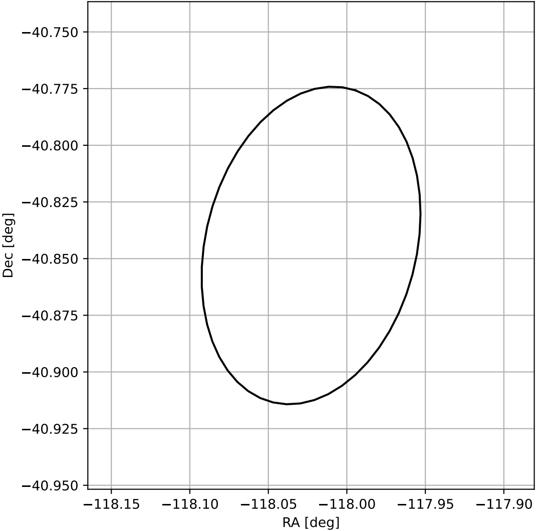
4FGL J1607.9-4050
