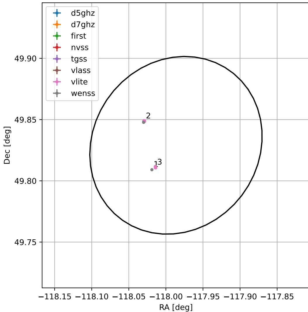
4FGL J1608.0+4949
