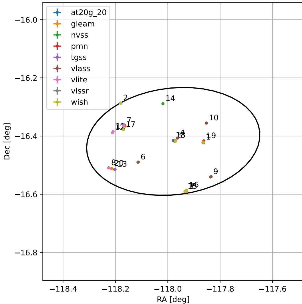
4FGL J1608.0-1625
