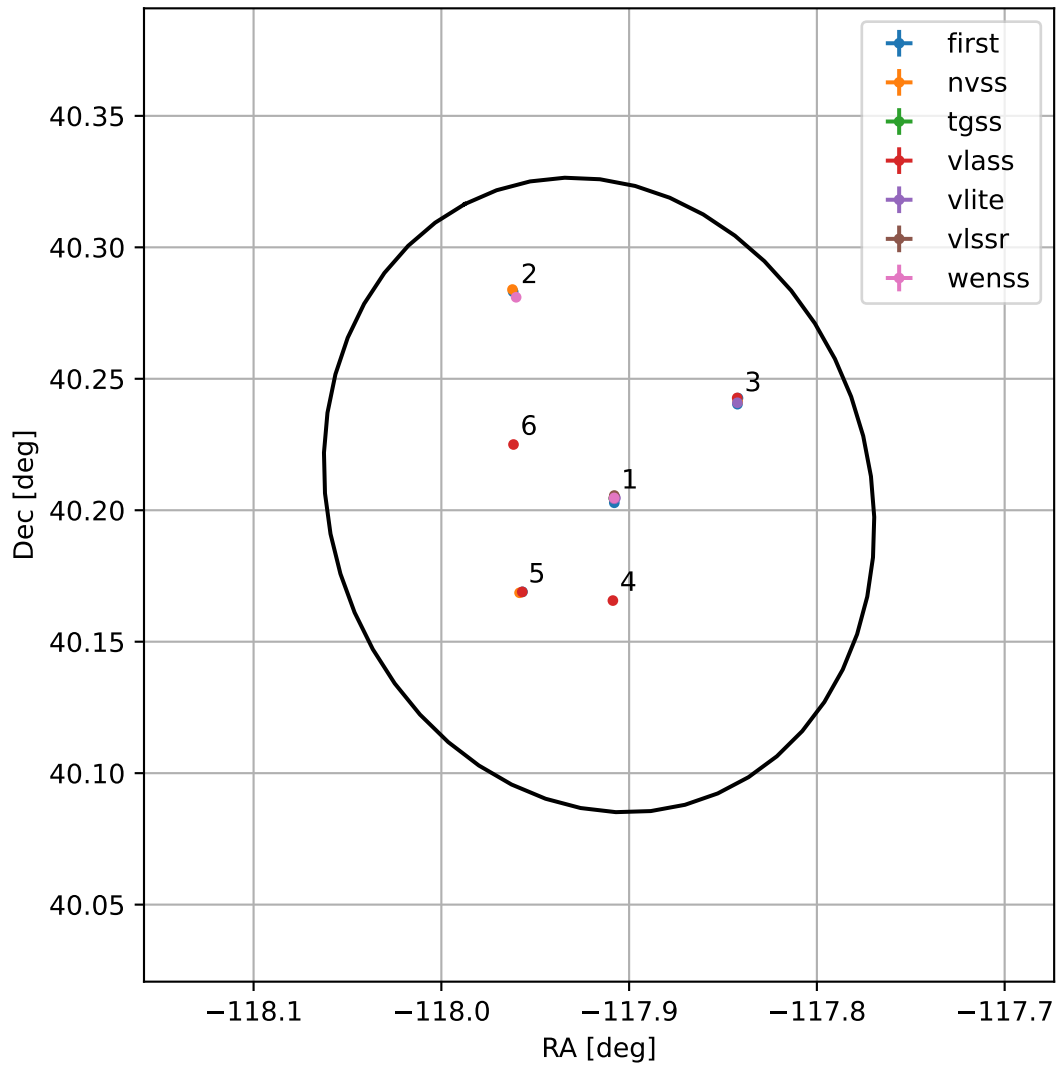
4FGL J1608.3+4012
