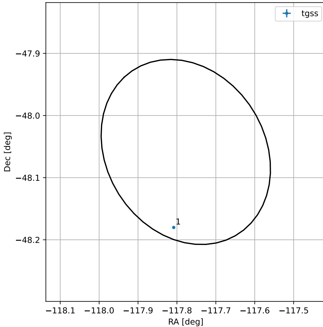
4FGL J1608.8-4803
