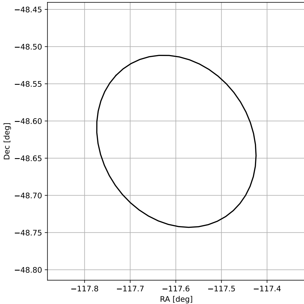
4FGL J1609.6-4837
