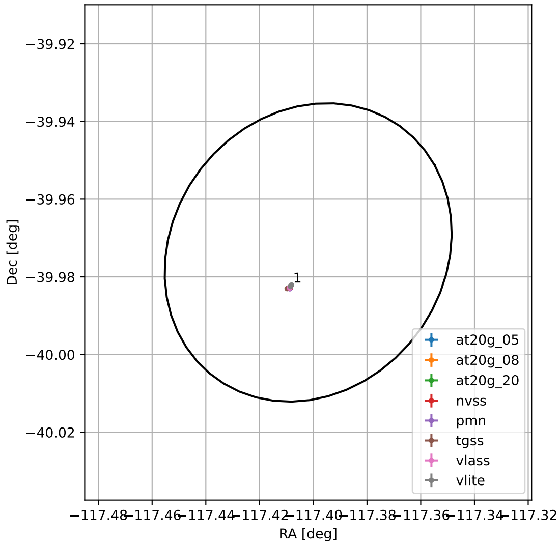
4FGL J1610.3-3958
