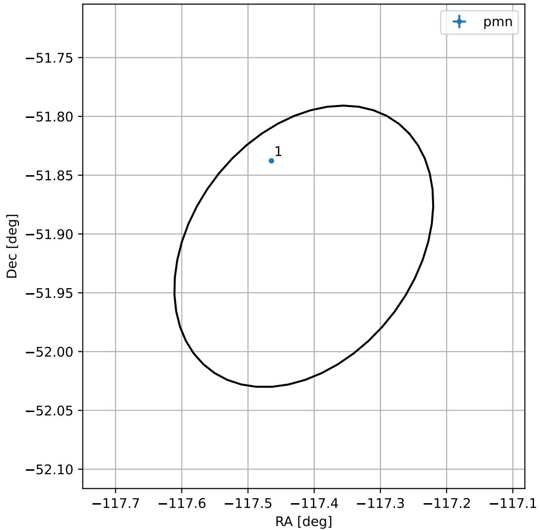
4FGL J1610.3-5154
