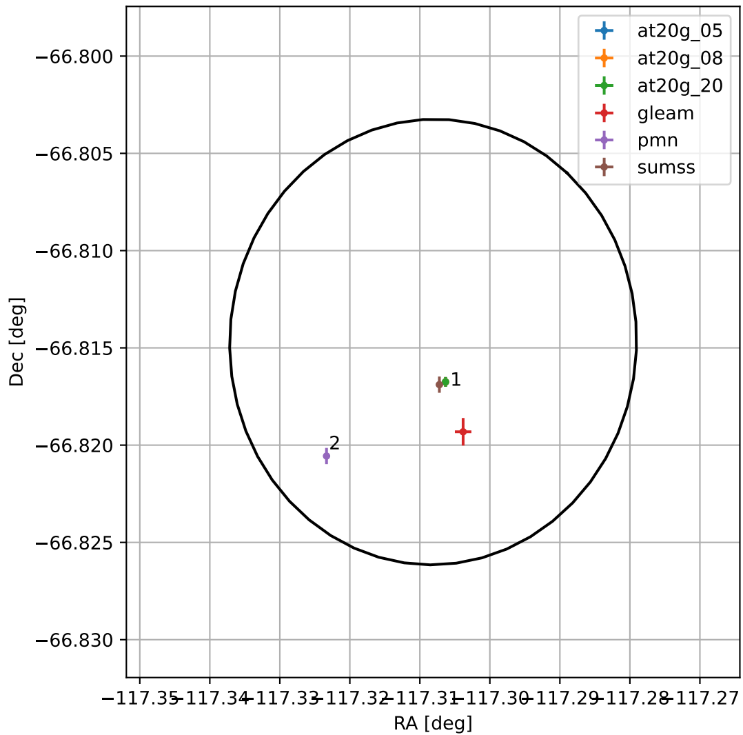
4FGL J1610.7-6648
