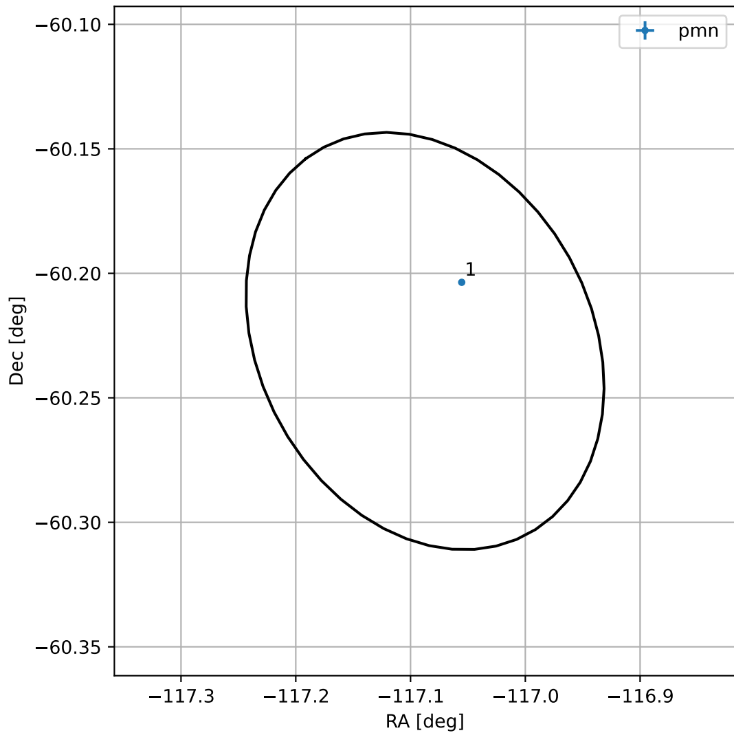
4FGL J1611.6-6013
