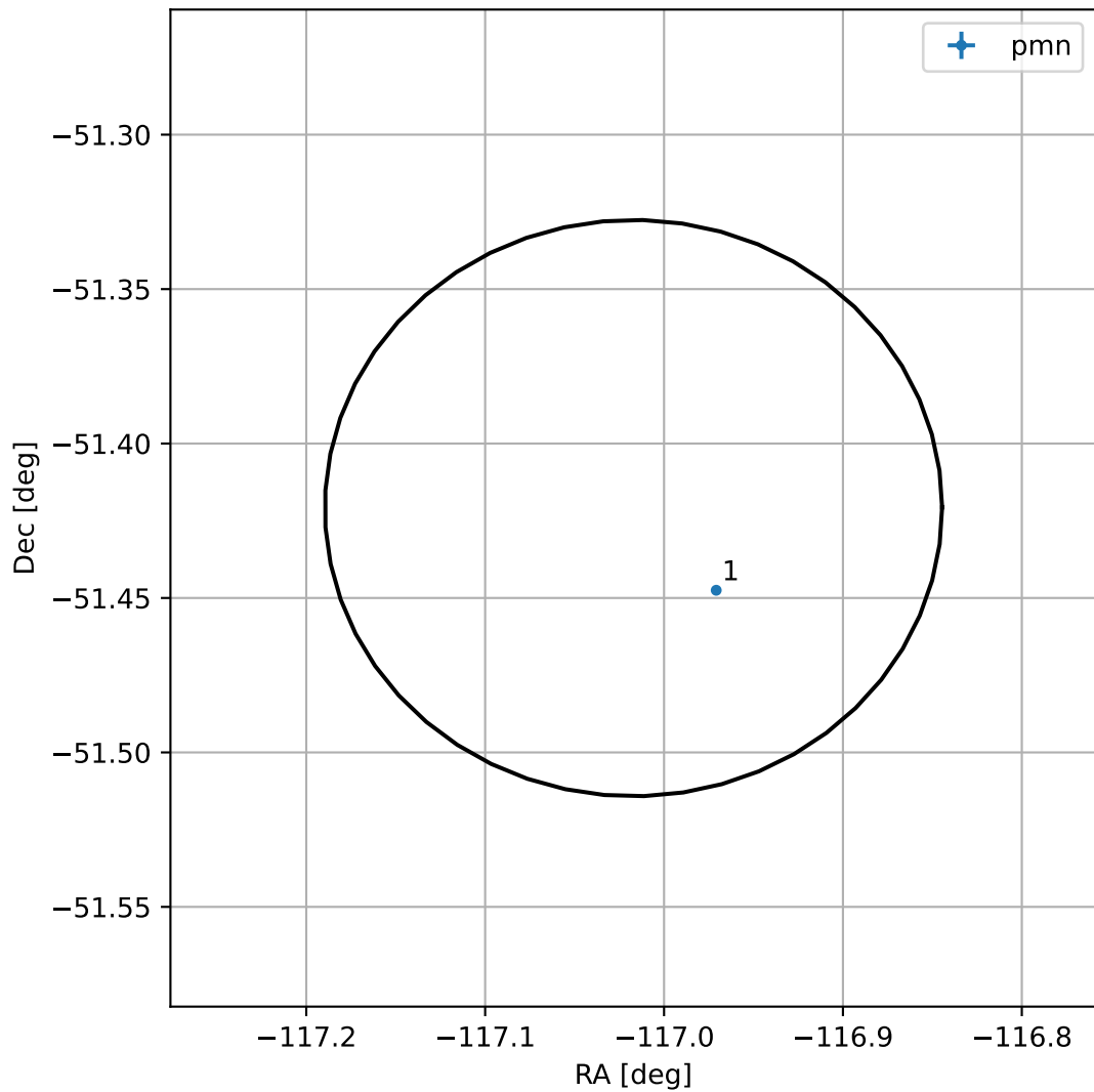
4FGL J1611.9-5125
