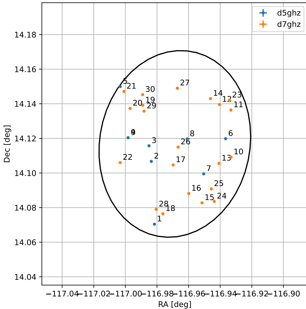
4FGL J1612.1+1407
