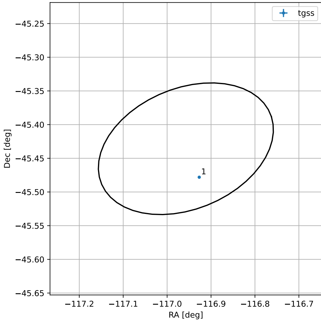
4FGL J1612.1-4526
