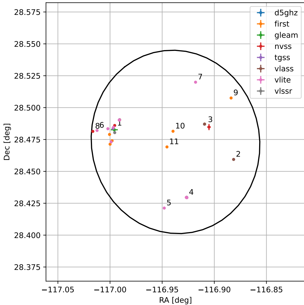
4FGL J1612.2+2828
