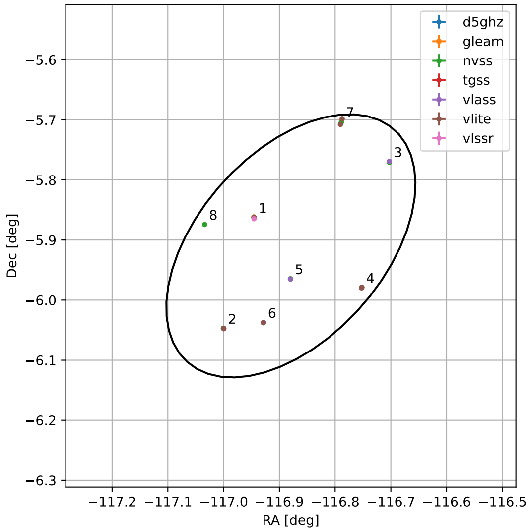
4FGL J1612.4-0554
