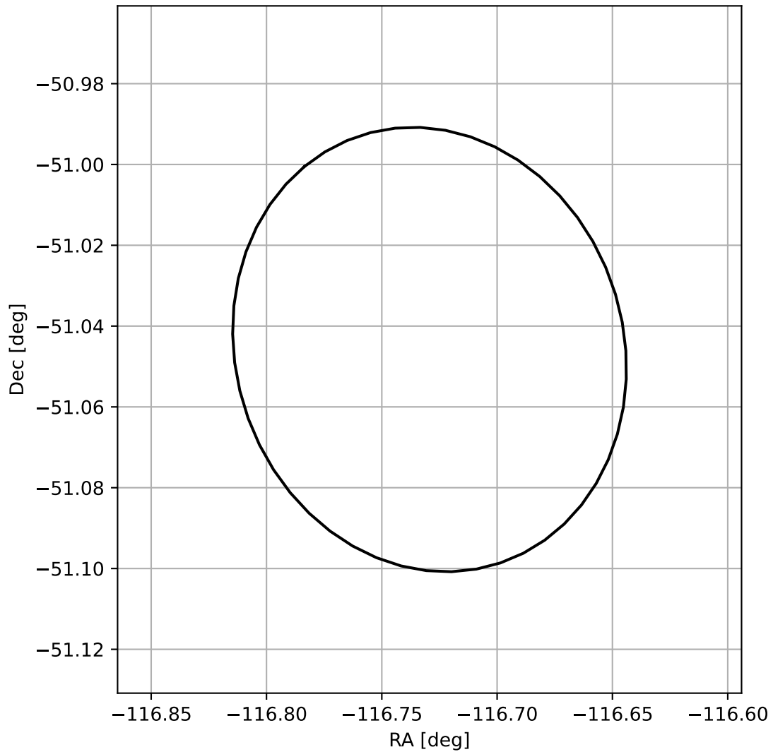
4FGL J1613.0-5102
