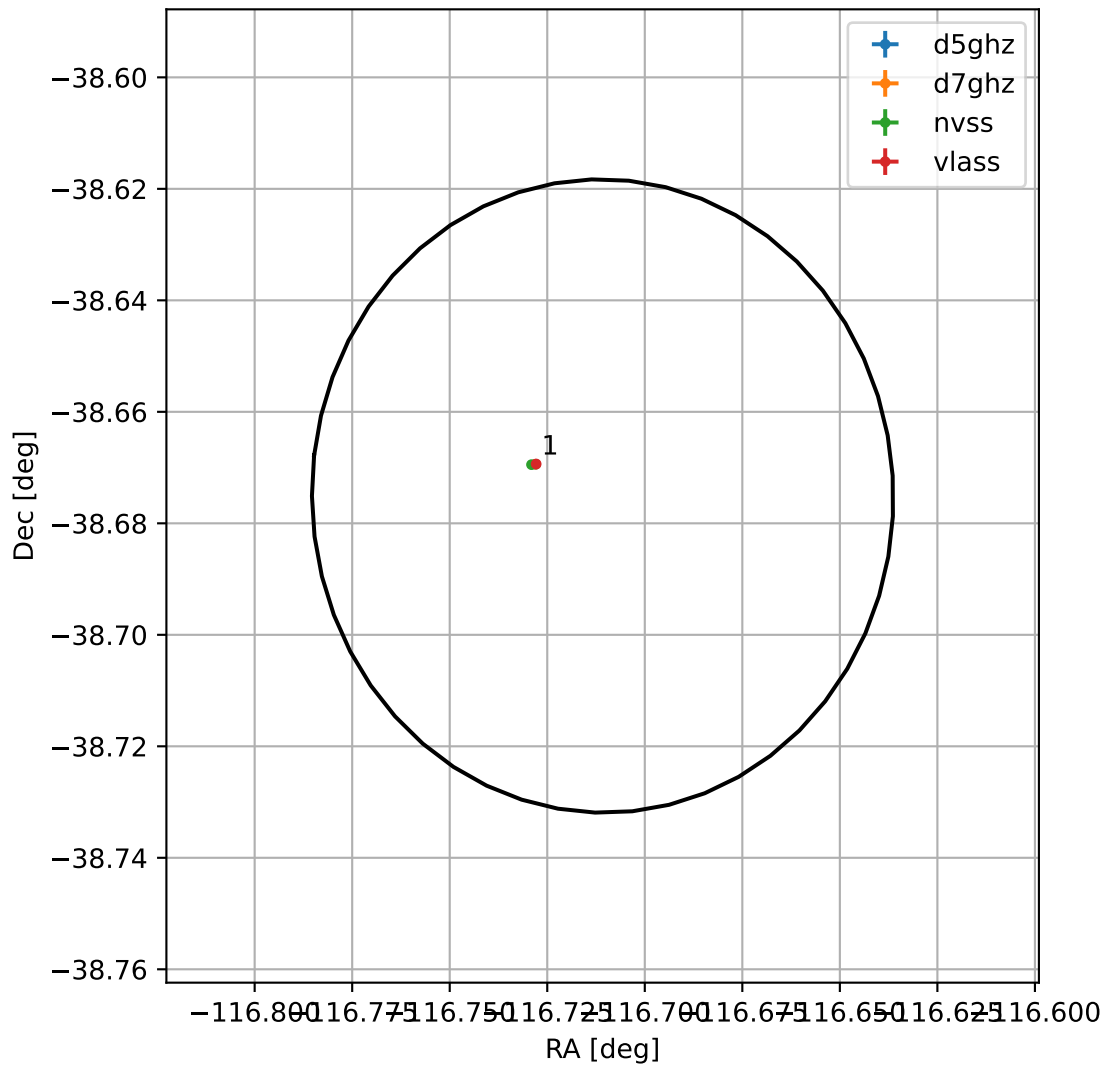
4FGL J1613.1-3840
