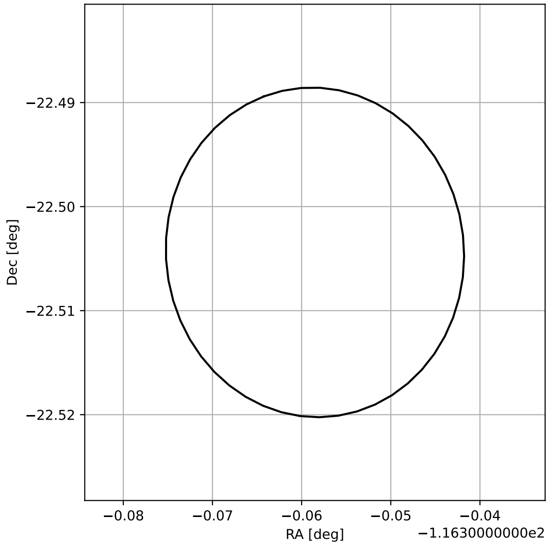
4FGL J1614.5-2230
