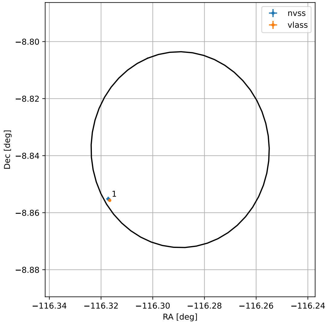
4FGL J1614.8-0850
