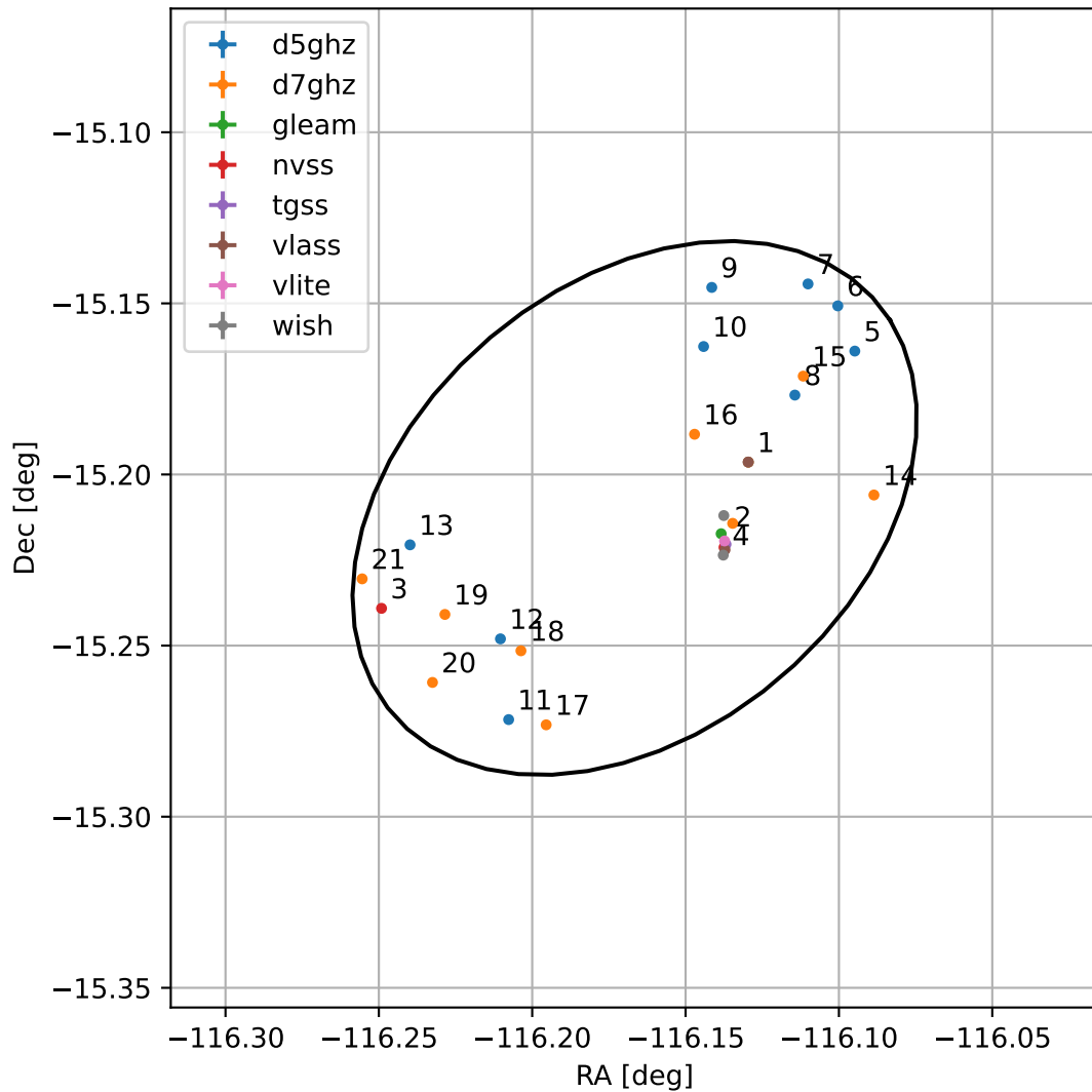
4FGL J1615.3-1512
