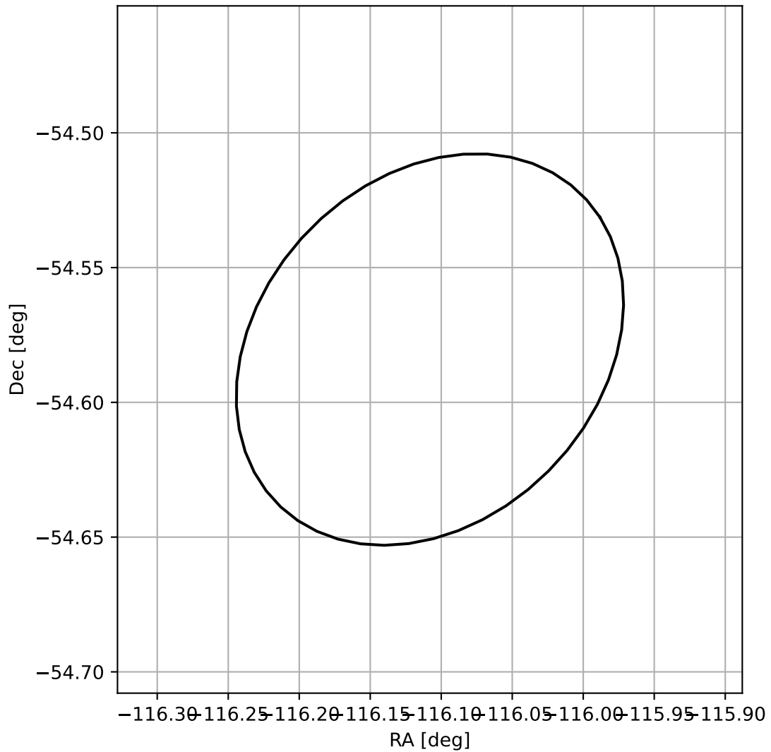
4FGL J1615.5-5434
