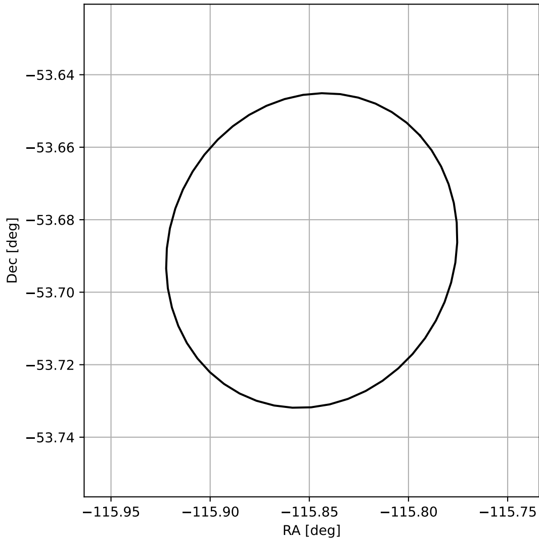
4FGL J1616.6-5341
