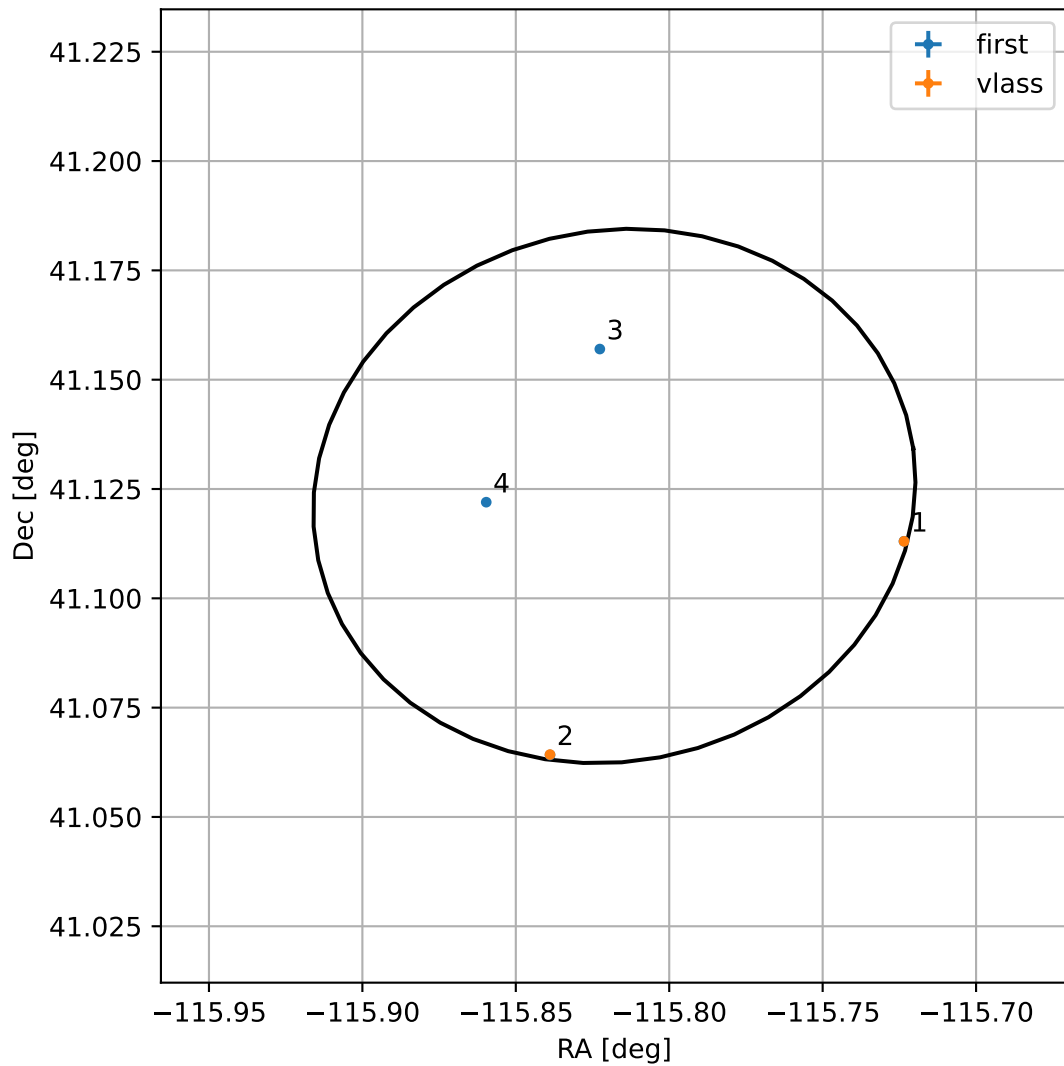
4FGL J1616.7+4107
