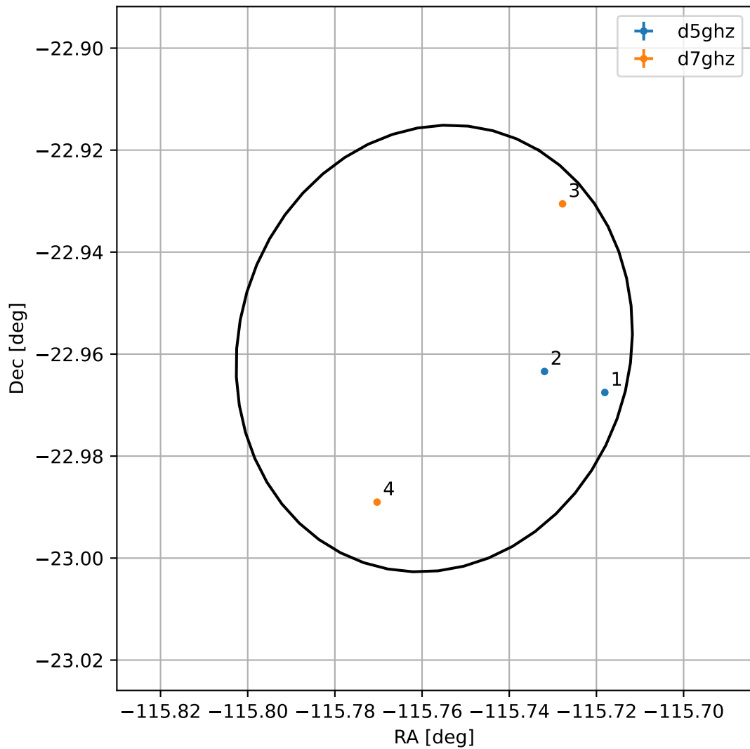
4FGL J1616.9-2257
