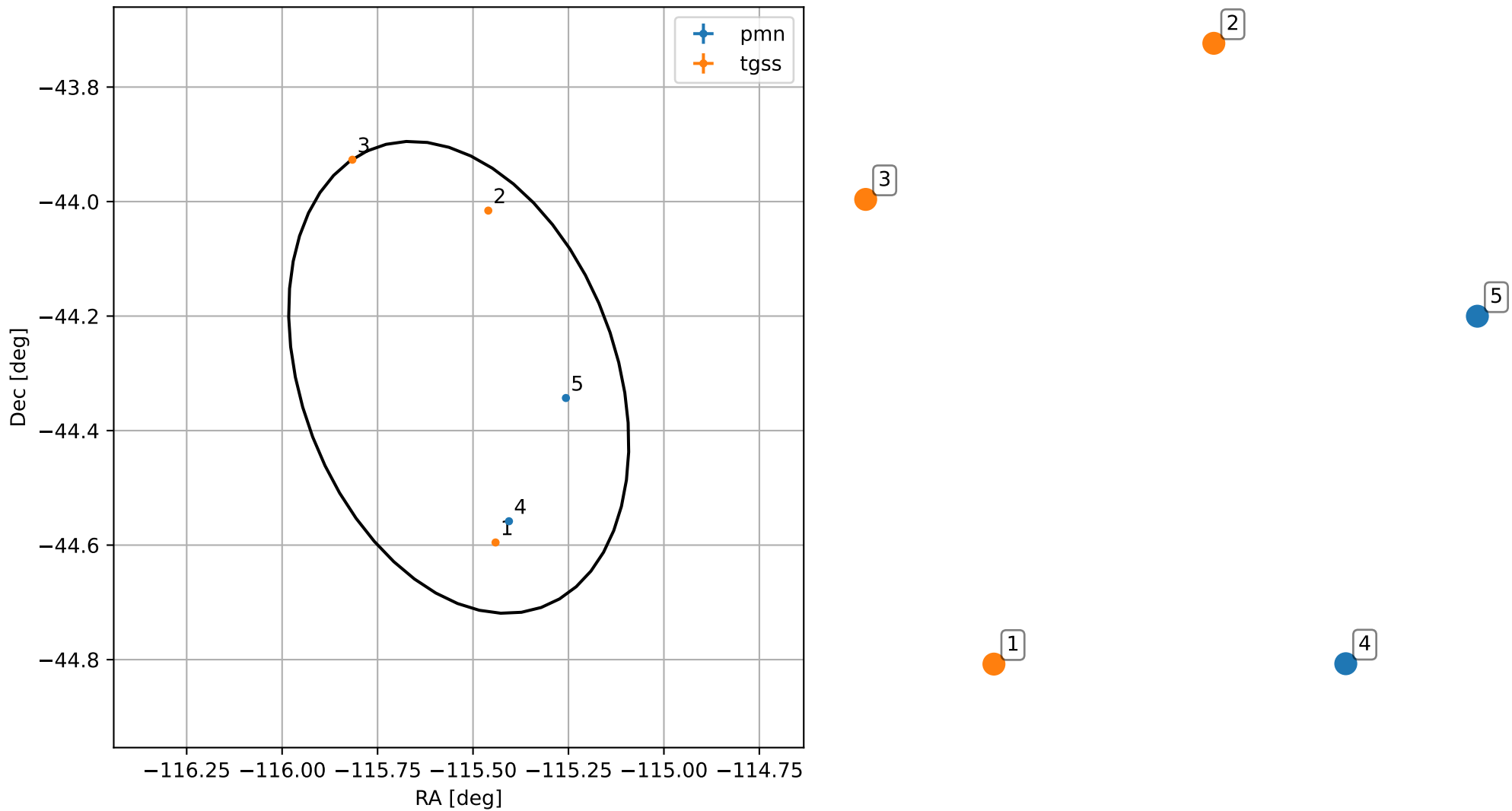
4FGL J1617.8-4418
