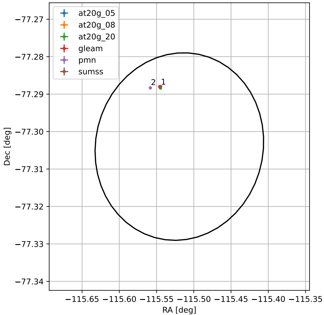
4FGL J1617.9-7718
