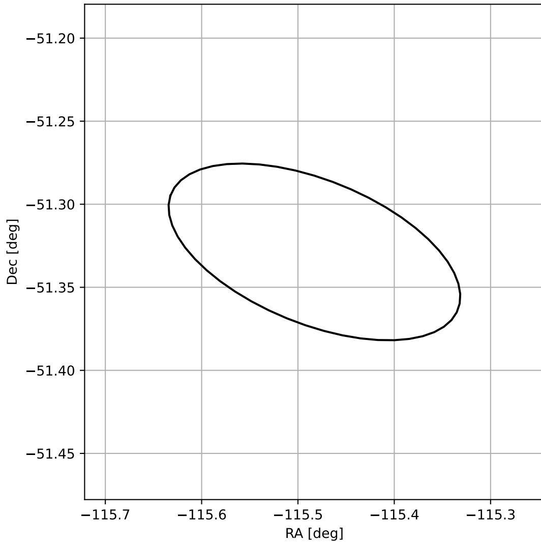
4FGL J1618.0-5119
