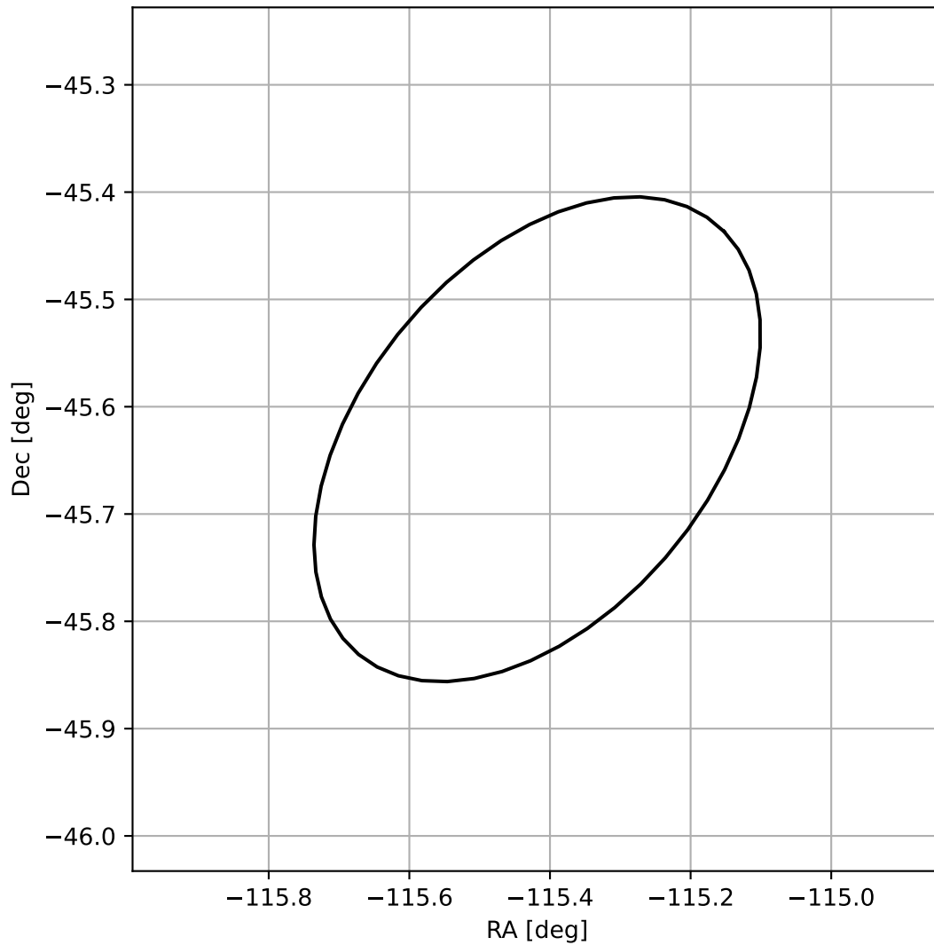
4FGL J1618.3-4537
