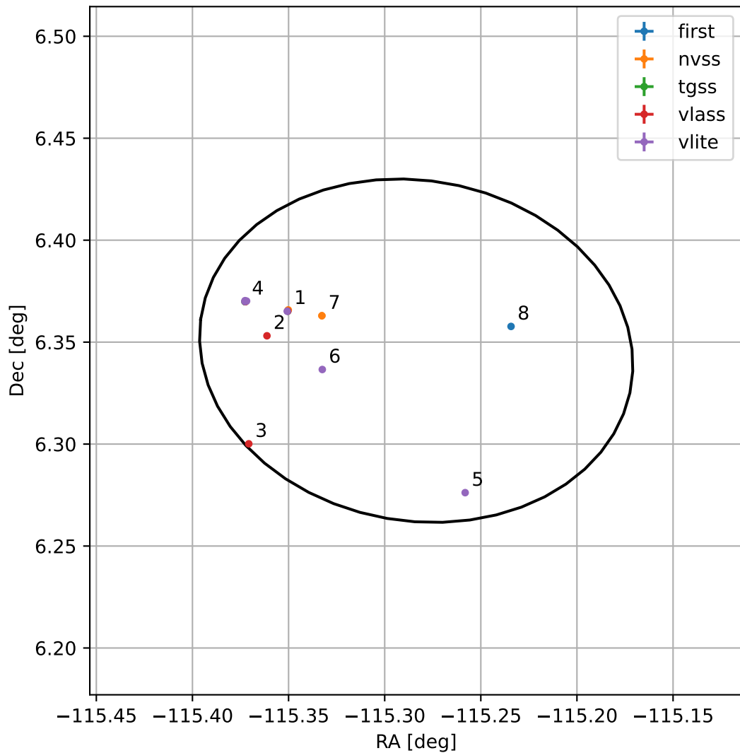
4FGL J1618.8+0620
