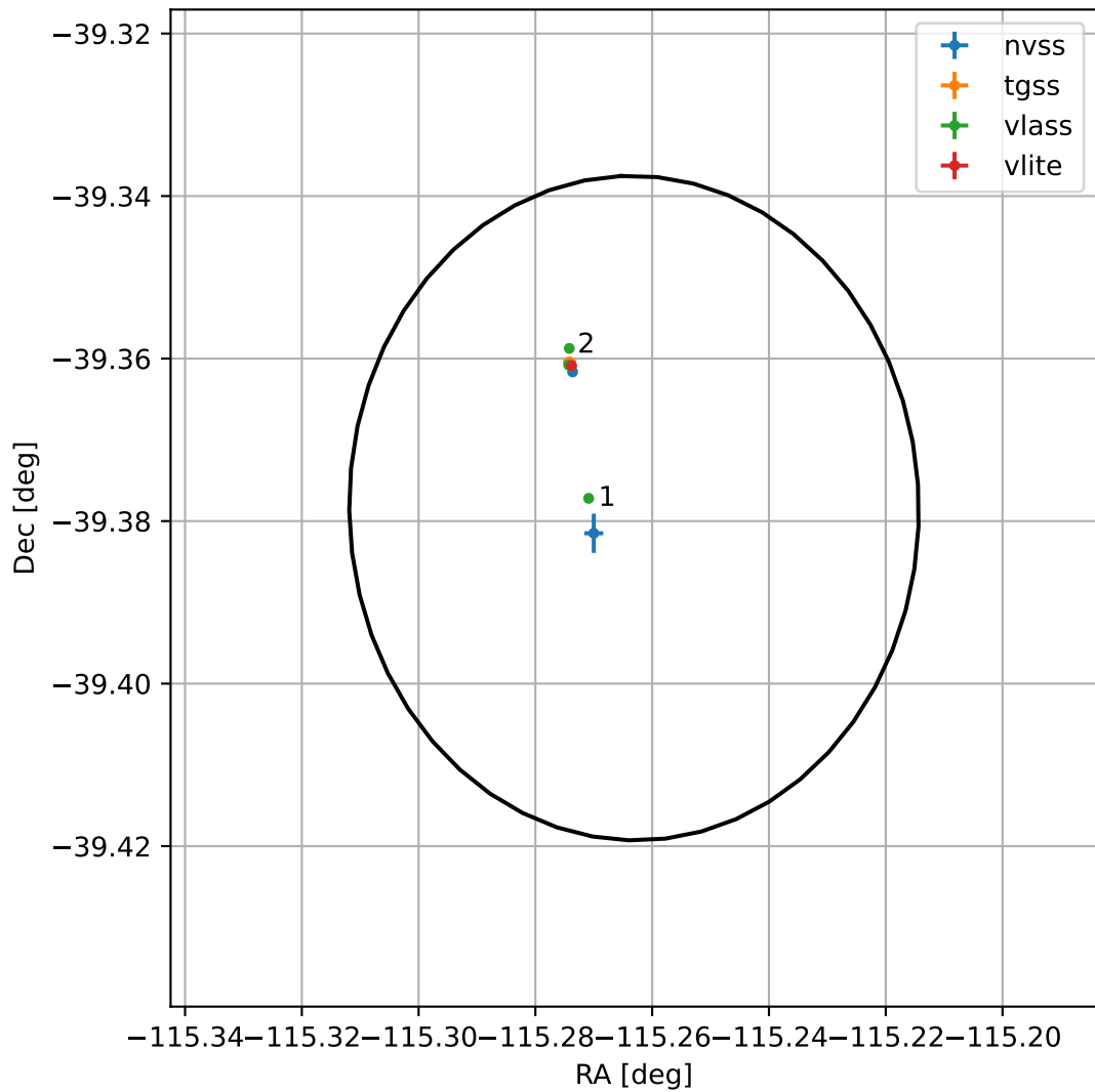
4FGL J1618.9-3922
