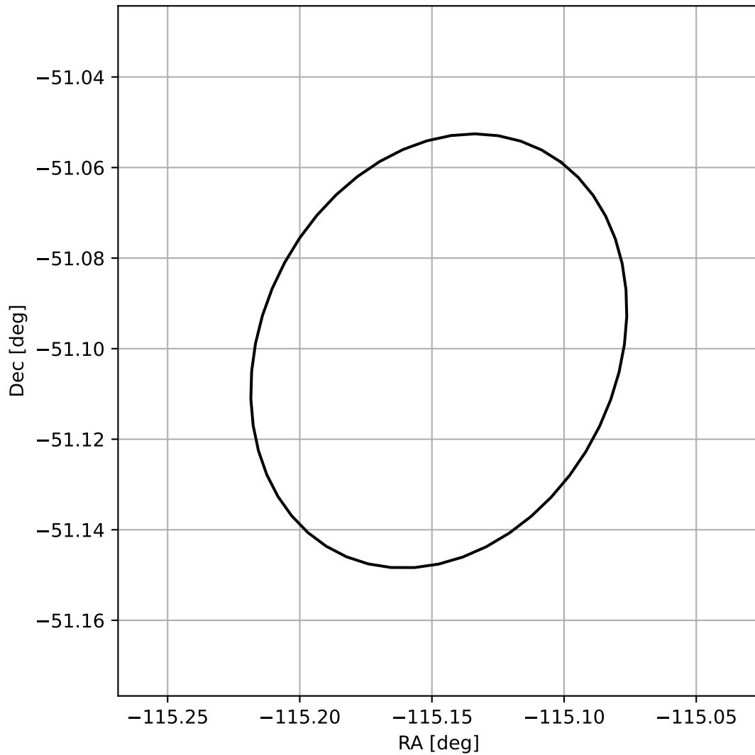
4FGL J1619.4-5106
