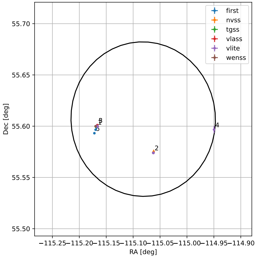
4FGL J1619.6+5536
