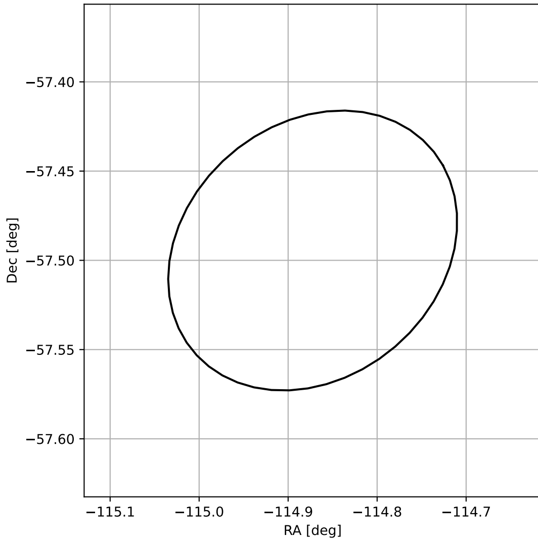
4FGL J1620.5-5729
